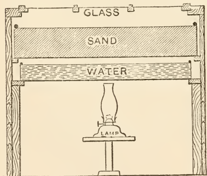
48. Simple propagating-oven.
